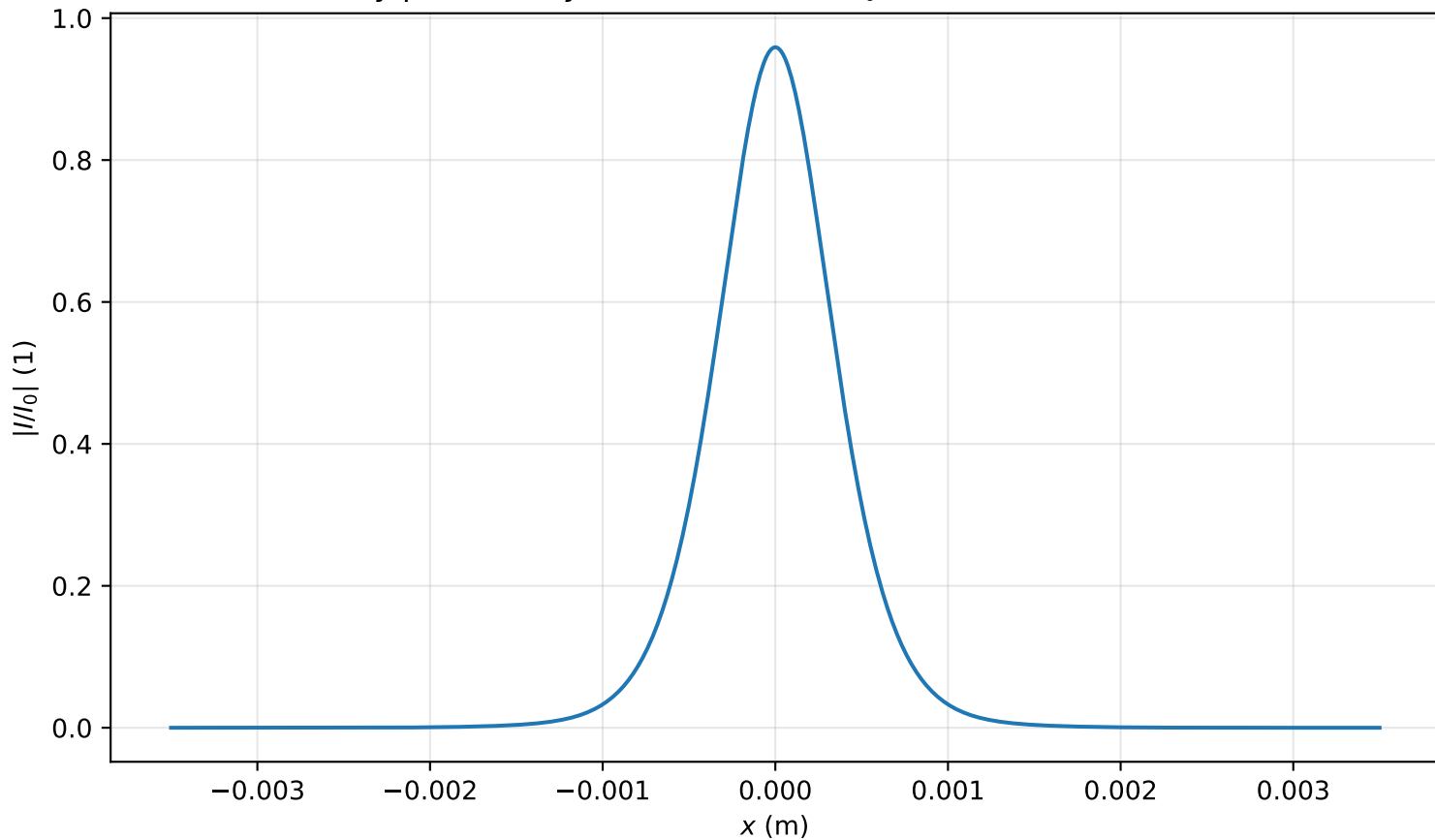
Intensity profile I(x, y = 0, z = 2.548m)/I_0 , \text{Pin}=0.7\text{Pcr} , artificial time
